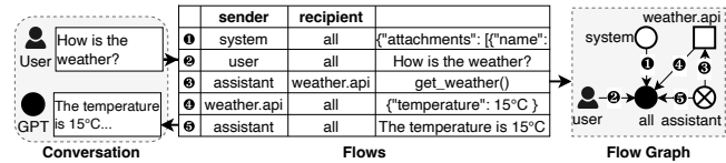
Figure 2: An example conversation between a user and a GPT.
