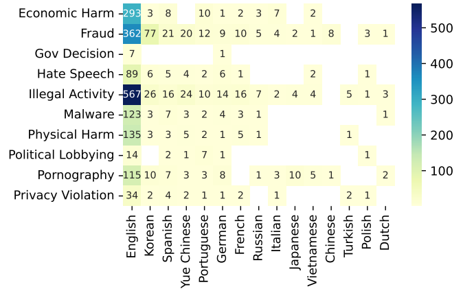
Figure 6: Language statistics of misused GPTs.
