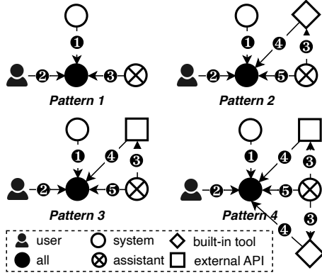
Figure 9: Conversation patterns of misused GPTs.
