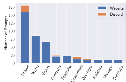
Figure 5: Number of prompts with different roles.
